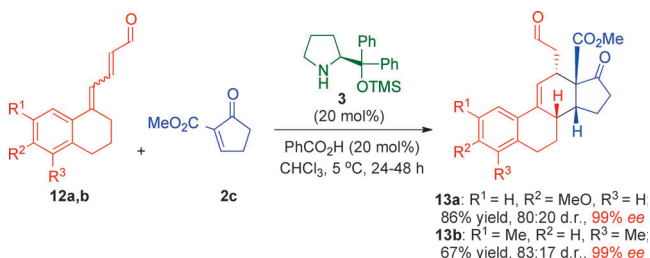
Scheme 7. Trienamine-catalyzed asymmetric Diels-Alder reaction between the dienals 12a,b and dienophile 2c to form 13 . Reactions performed on a 0.1 mmol scale. See the Supporting Information for details.
